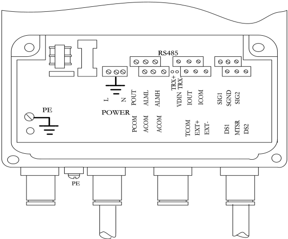
Fig.4.3 (a) Connectors for 211B
